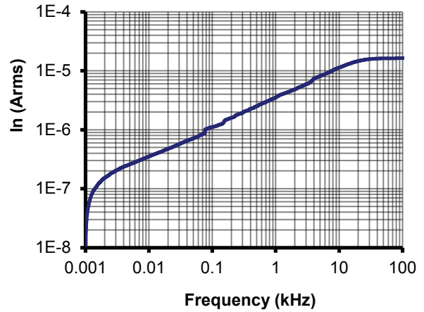
Figure 14: Typical total output current noise (rms) with R_M = 50 \Omega ( f_c is upper cut-off frequency of bandpass, low cut off frequency is 1 Hz)
