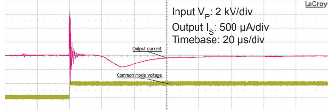
Figure 12: Detail of typical common mode perturbation (2000 V step with 6 kV/μs, R_M = 100 \Omega )
