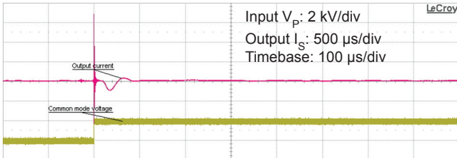
Figure 11: Typical common mode perturbation (2000 V step with 6 kV/μs R_M = 100 \Omega )
